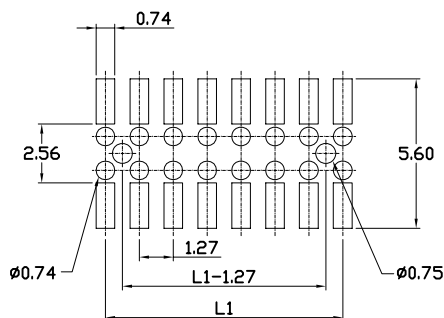
RECOMMENDED P.C.B. SMT LAYOUT TOLERANCE \pm 0.05
